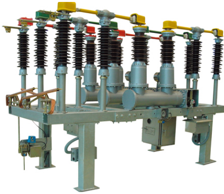
SF6 ZCW10-40.5G (Hybrid Compact Switchgear Assembly)
